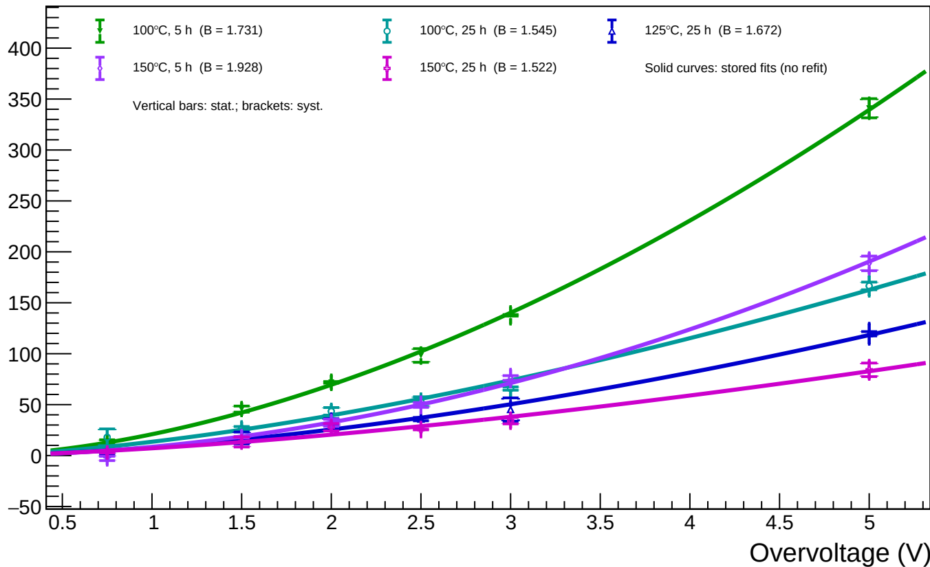
B1_T=20 - Spot 83 (x = 1465.19, y = 152.51): luminosity vs overvoltage for all annealing phases
