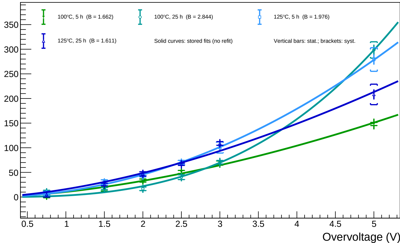
B1_T=20 - Spot 84 (x = 1744.36, y = 665.05): luminosity vs overvoltage for all annealing phases
