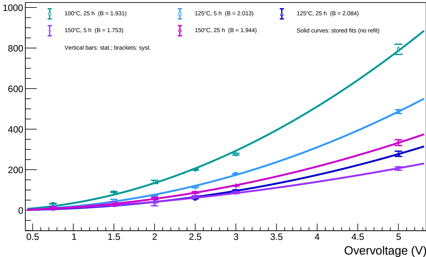
B1_T=20 - Spot 85 ( x = 194.64 , y = 135.03 ): luminosity vs overvoltage for all annealing phases
