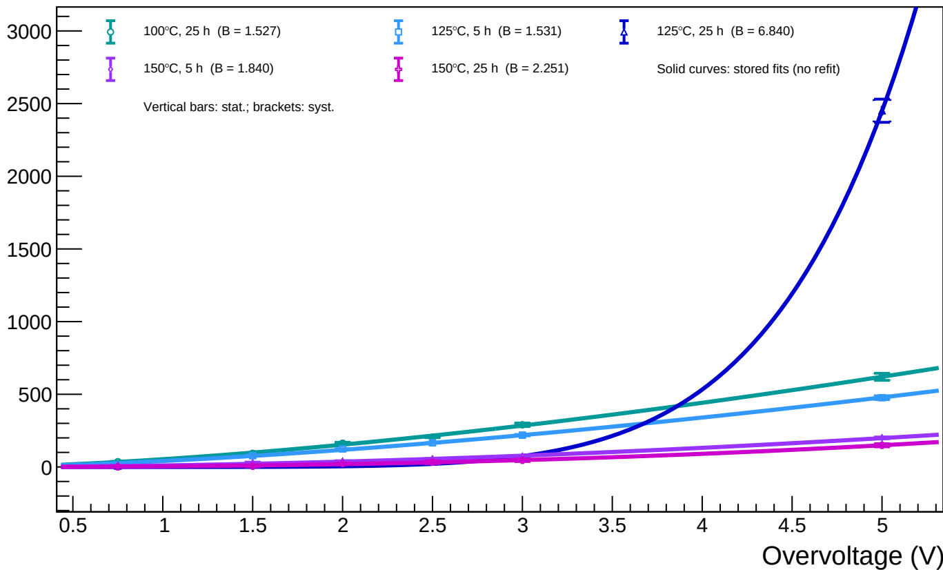
B1_T=20 - Spot 87 ( x = 258.52 , y = 134.94 ): luminosity vs overvoltage for all annealing phases
