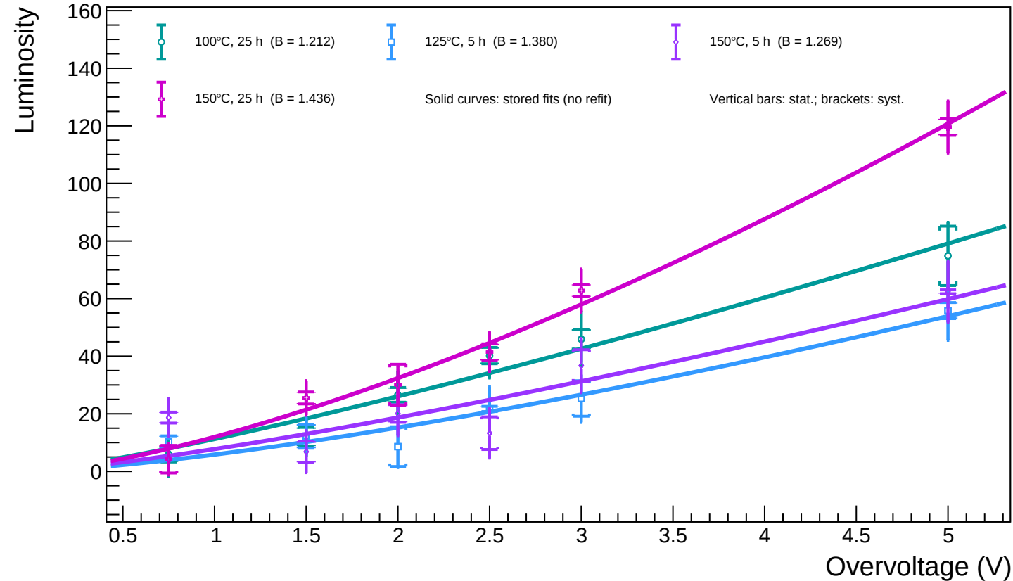
B1_T=20 - Spot 88 (x = 371.29, y = 1003.93): luminosity vs overvoltage for all annealing phases
