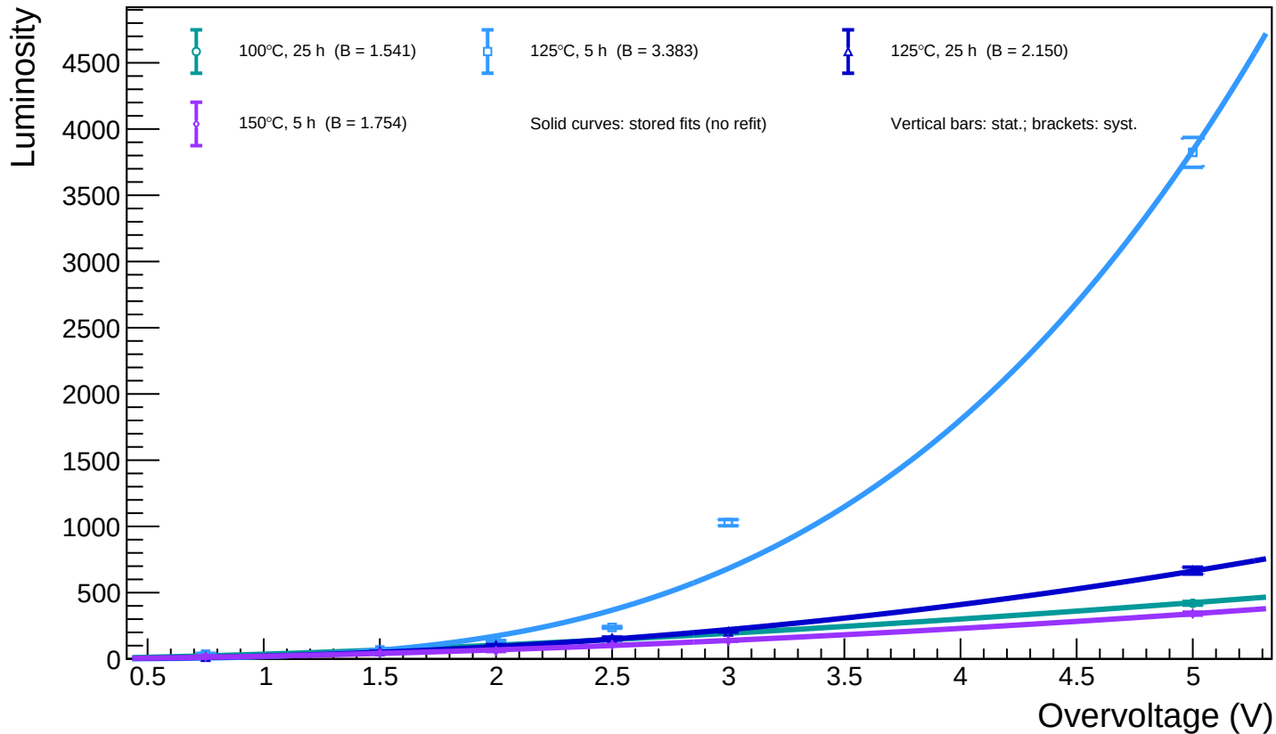
B1_T=20 - Spot 89 ( x = 562.30 , y = 288.42 ): luminosity vs overvoltage for all annealing phases
