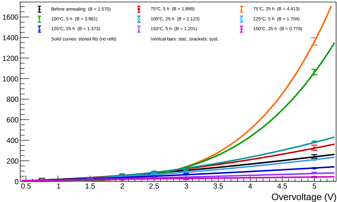
B1_T=20 - Spot 9 (x = 316.41, y = 878.52): luminosity vs overvoltage for all annealing phases
