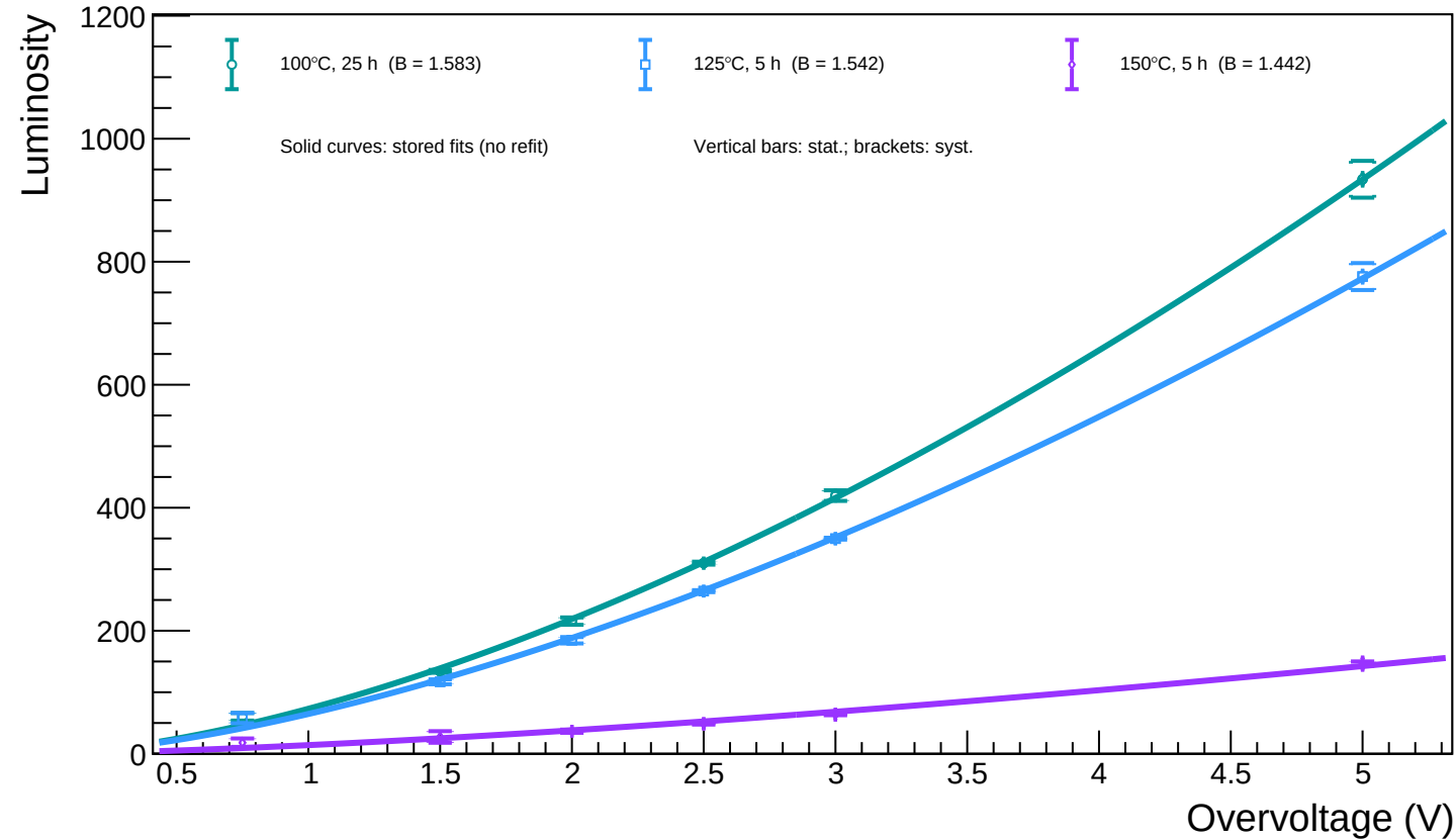
B1_T=20 - Spot 90 ( x = 744.94 , y = 905.79 ): luminosity vs overvoltage for all annealing phases
