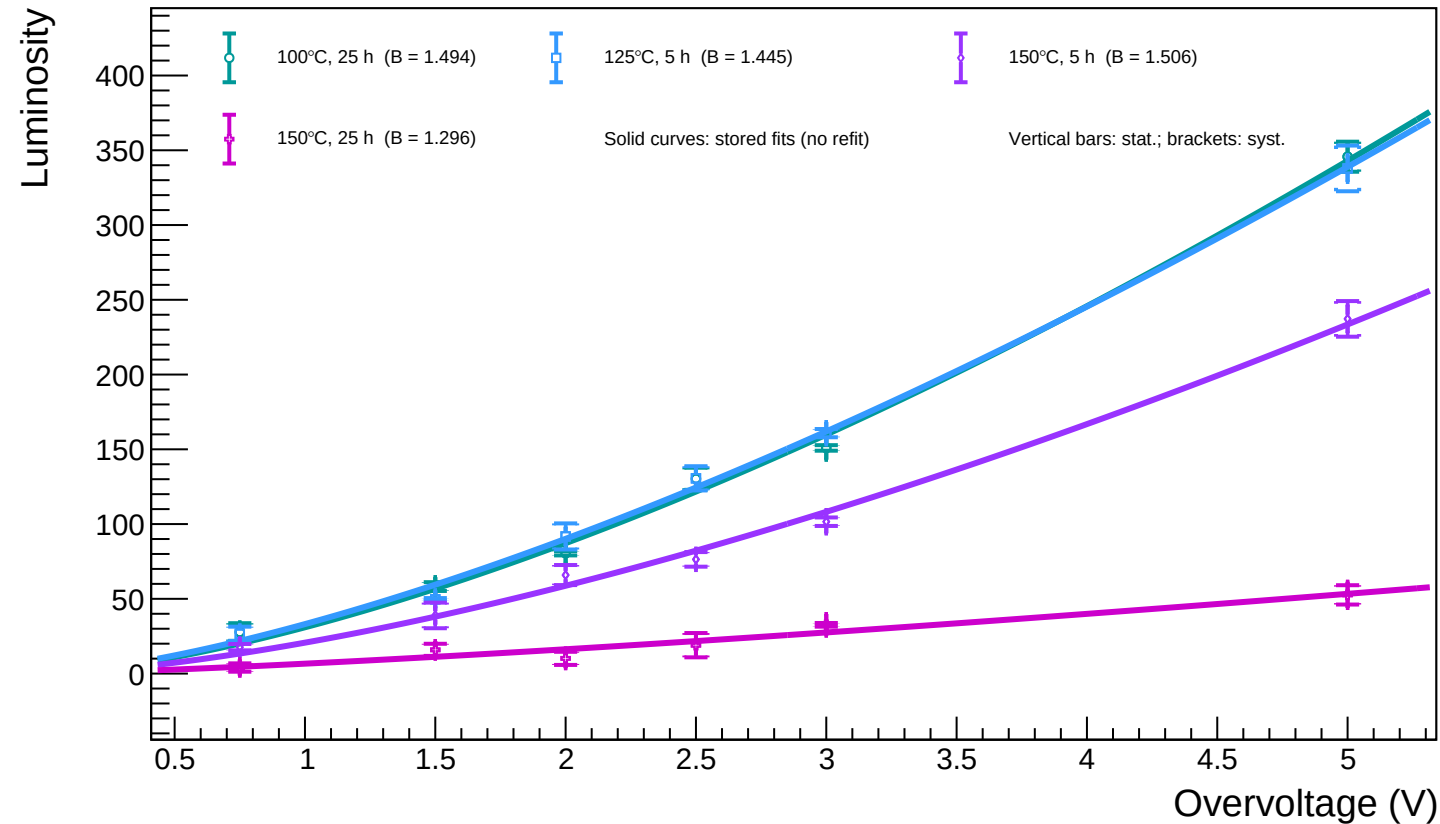
B1_T=20 - Spot 91 ( x = 788.90 , y = 989.47 ): luminosity vs overvoltage for all annealing phases
