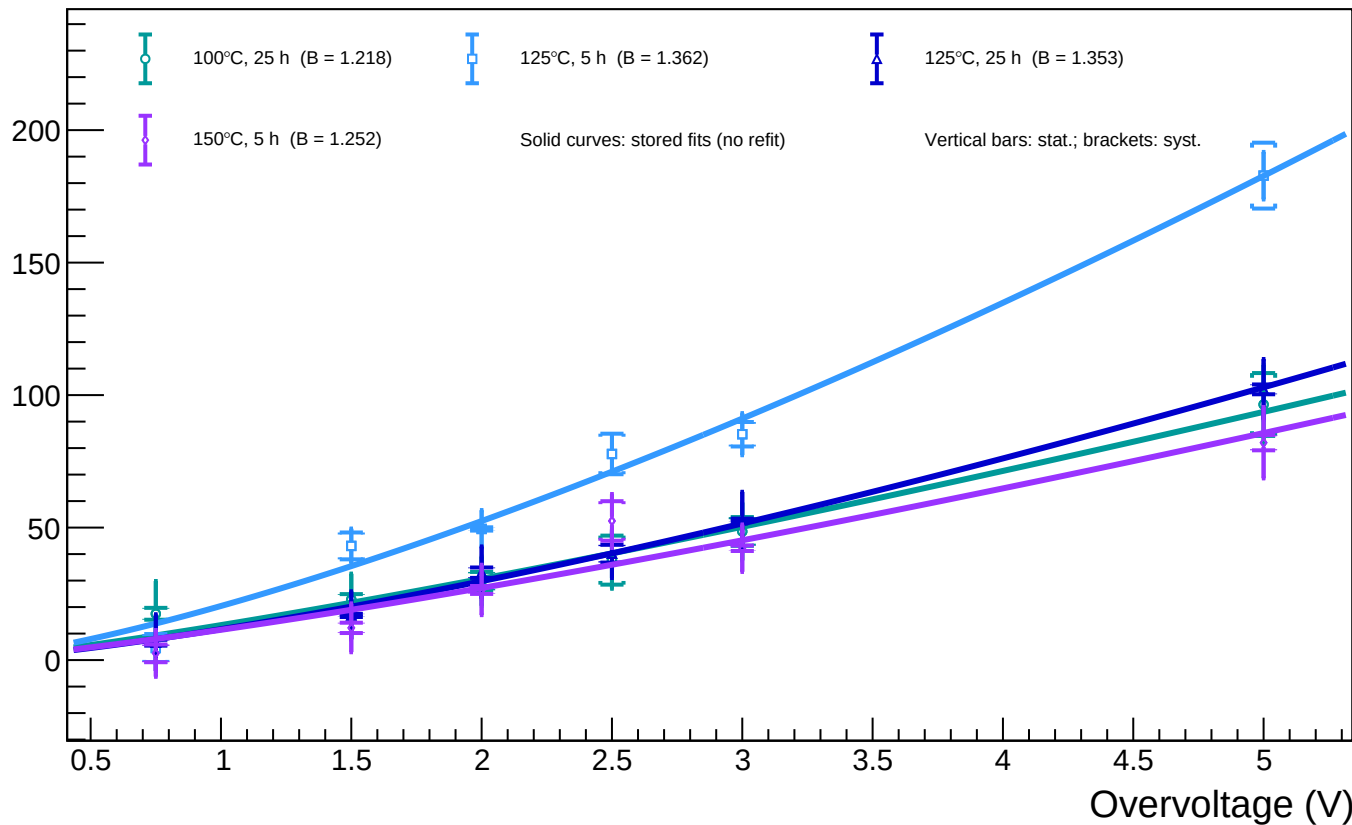
B1_T=20 - Spot 92 (x = 1093.70, y = 324.55): luminosity vs overvoltage for all annealing phases
