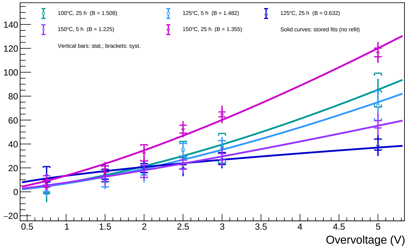
B1_T=20 - Spot 94 (x = 1482.38, y = 788.35): luminosity vs overvoltage for all annealing phases
