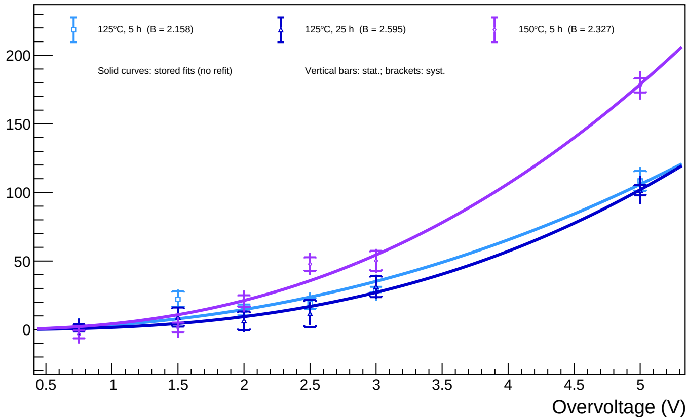
B1_T=20 - Spot 98 ( x = 929.99 , y = 208.16 ): luminosity vs overvoltage for all annealing phases
