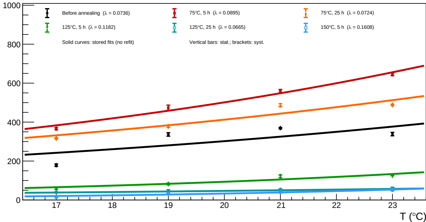
B1_v=3 - Spot 0 (x = 79.71, y = 333.69): luminosity vs temperature for all annealing phases
