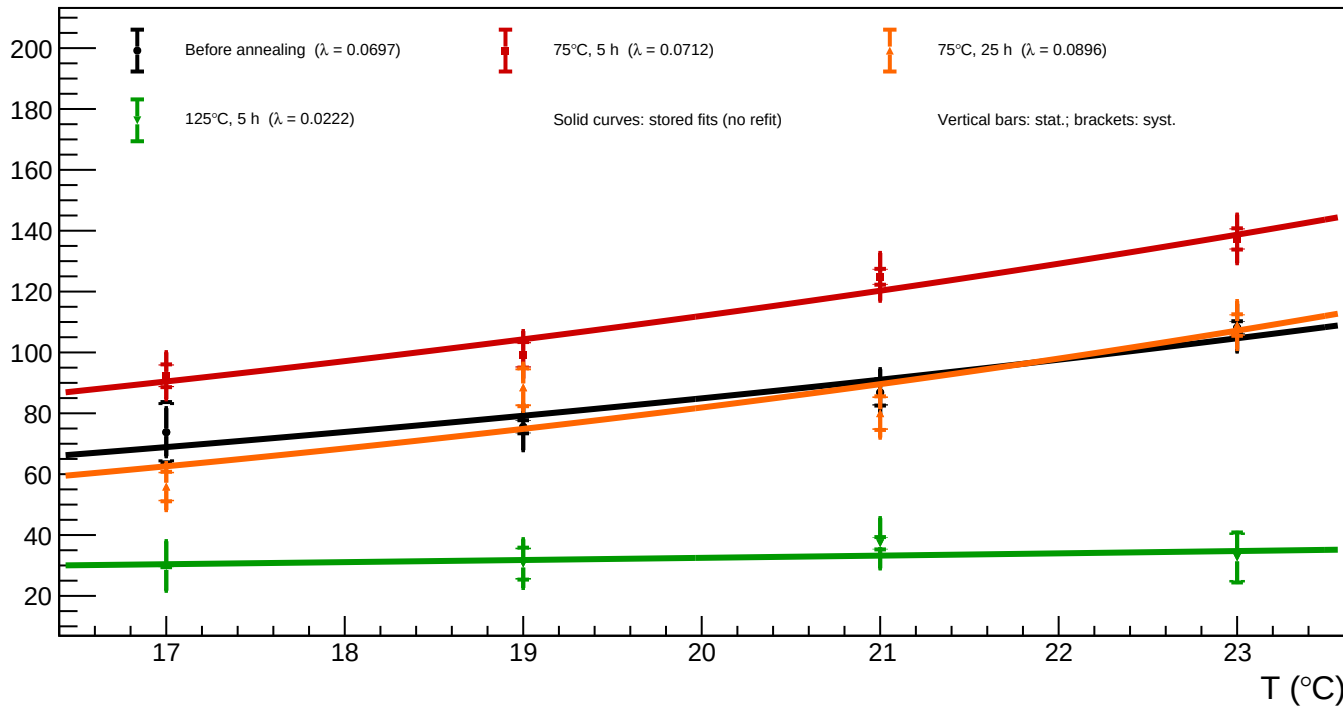
B1_v=3 - Spot 1 (x = 89.15, y = 699.39): luminosity vs temperature for all annealing phases
