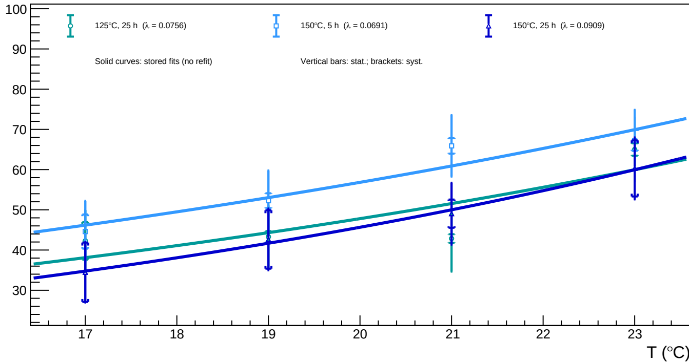
B1_v=3 - Spot 100 (x = 1565.37, y = 884.90): luminosity vs temperature for all annealing phases
