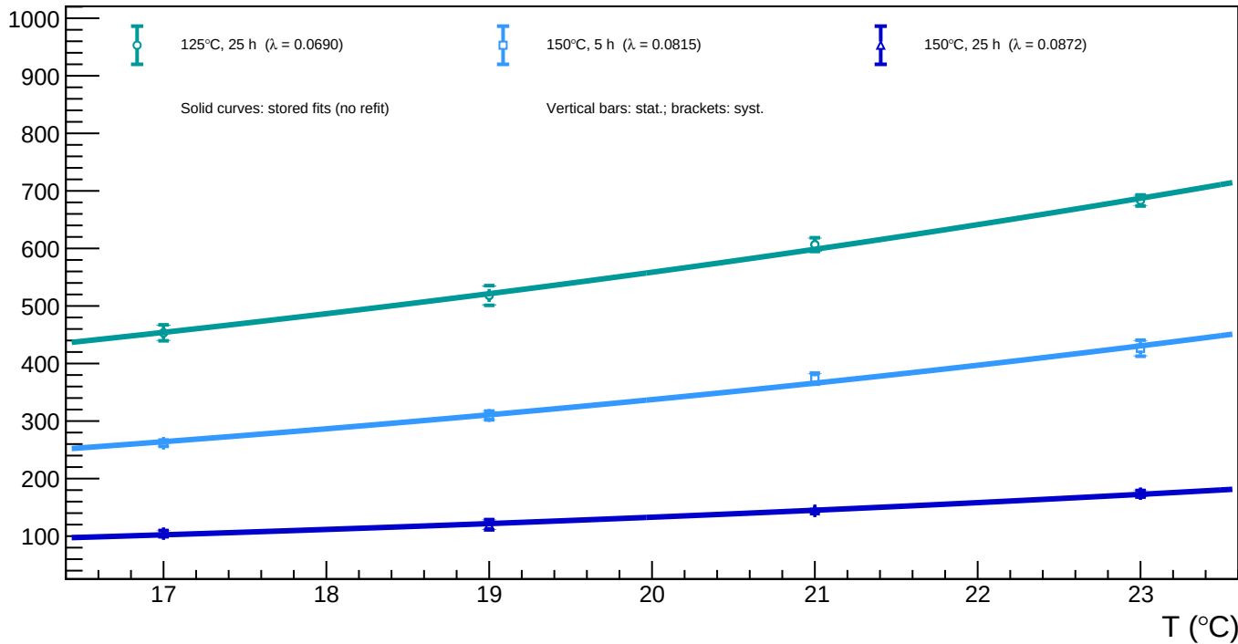
B1_v=3 - Spot 101 (x = 1603.93, y = 810.31): luminosity vs temperature for all annealing phases
