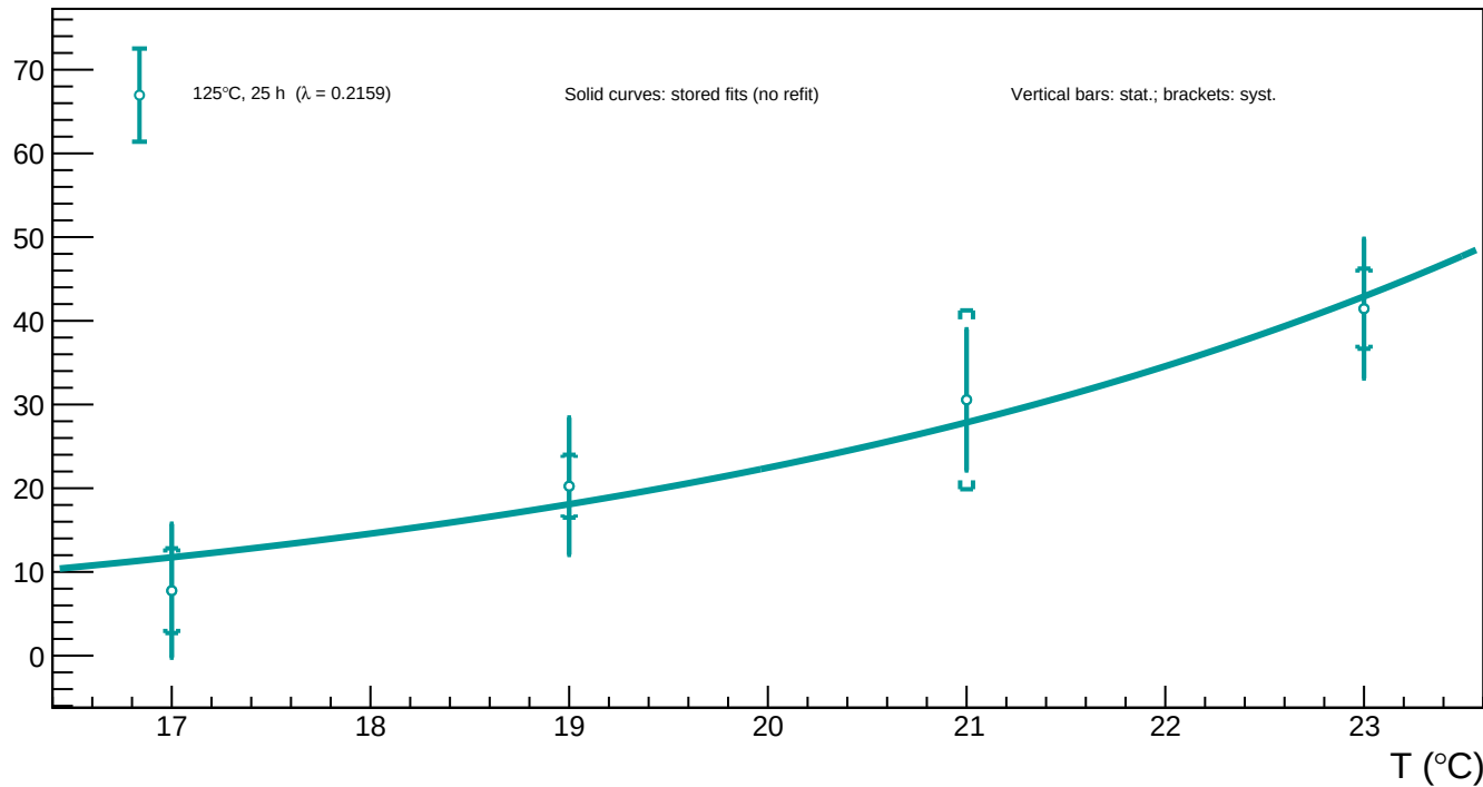
B1_v=3 - Spot 103 ( x = 409.92 , y = 210.73 ): luminosity vs temperature for all annealing phases
