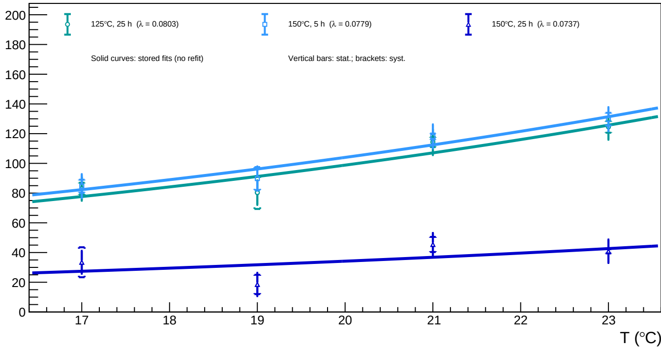
B1_v=3 - Spot 107 (x = 1625.74, y = 629.55): luminosity vs temperature for all annealing phases
