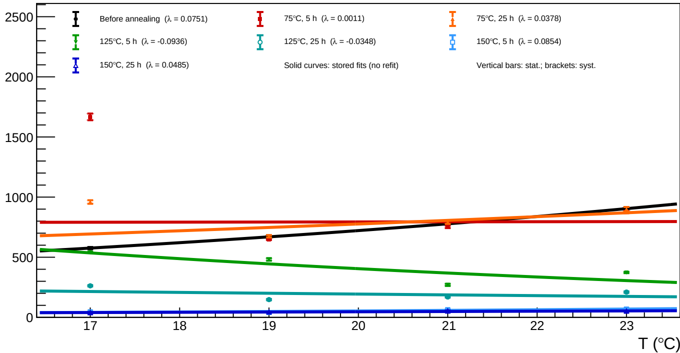
B1_v=3 - Spot 11 (x = 346.30, y = 551.07): luminosity vs temperature for all annealing phases
