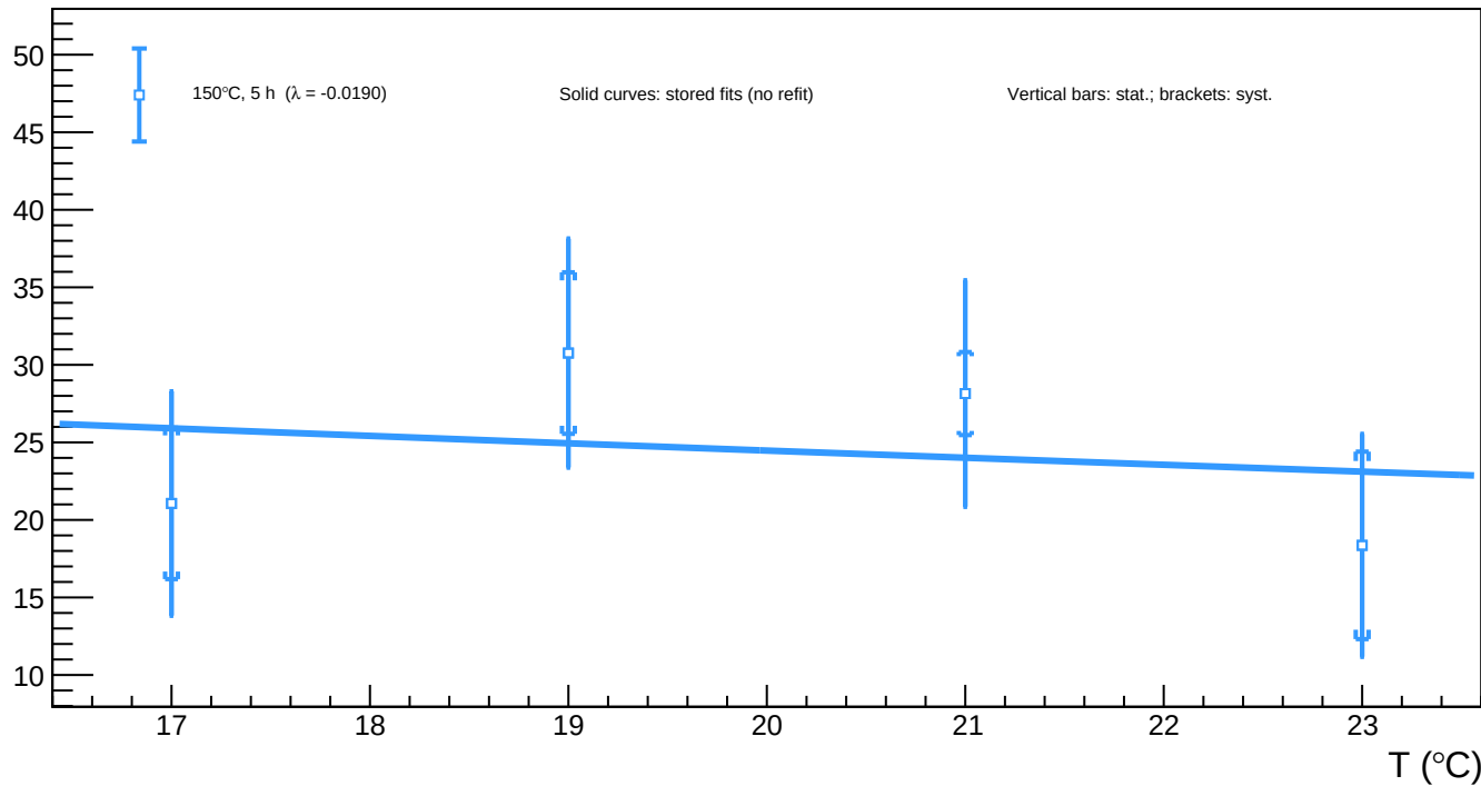
B1_v=3 - Spot 115 ( x = 520.13 , y = 918.45 ): luminosity vs temperature for all annealing phases
