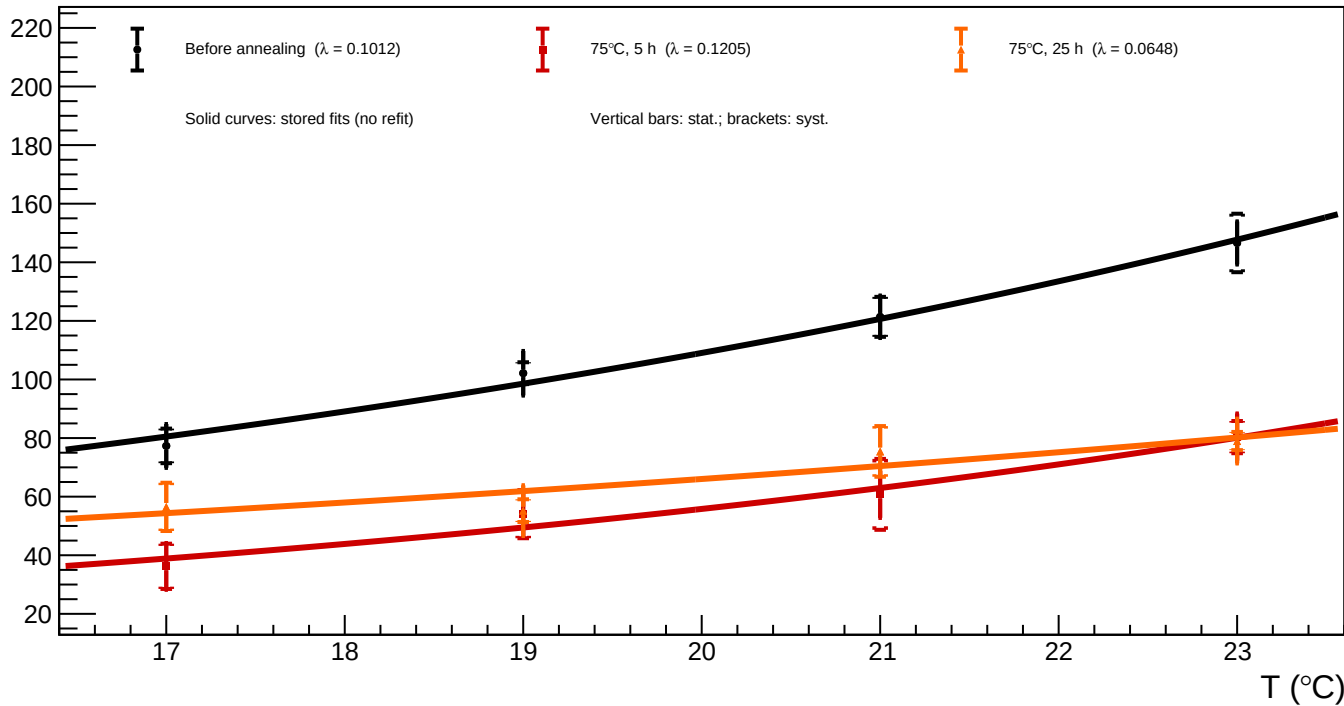
B1_v=3 - Spot 13 (x = 349.81, y = 707.16): luminosity vs temperature for all annealing phases
