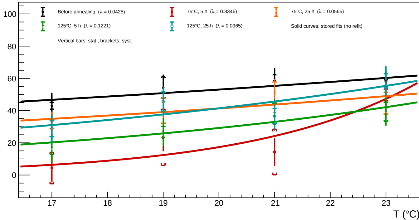
B1_v=3 - Spot 15 (x = 404.62, y = 526.59): luminosity vs temperature for all annealing phases
