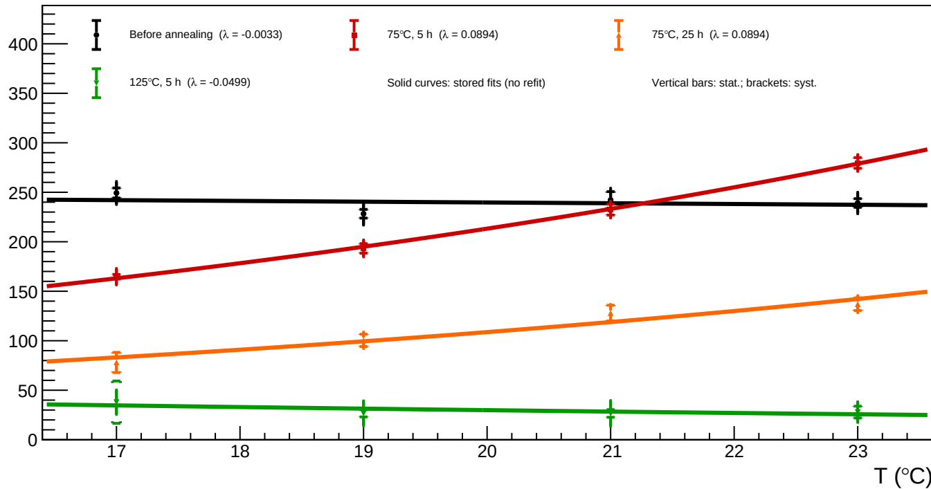
B1_v=3 - Spot 17 (x = 456.94, y = 886.03): luminosity vs temperature for all annealing phases
