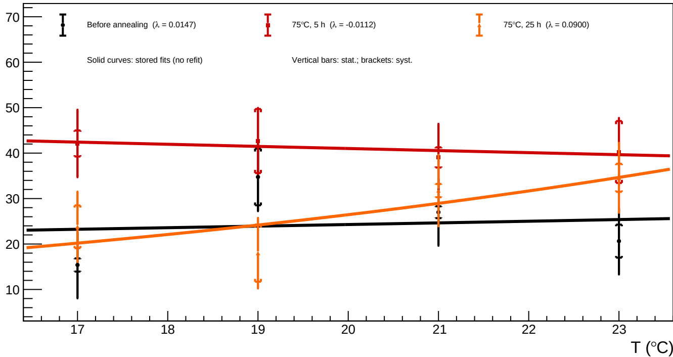
B1_v=3 - Spot 19 (x = 489.19, y = 666.03): luminosity vs temperature for all annealing phases
