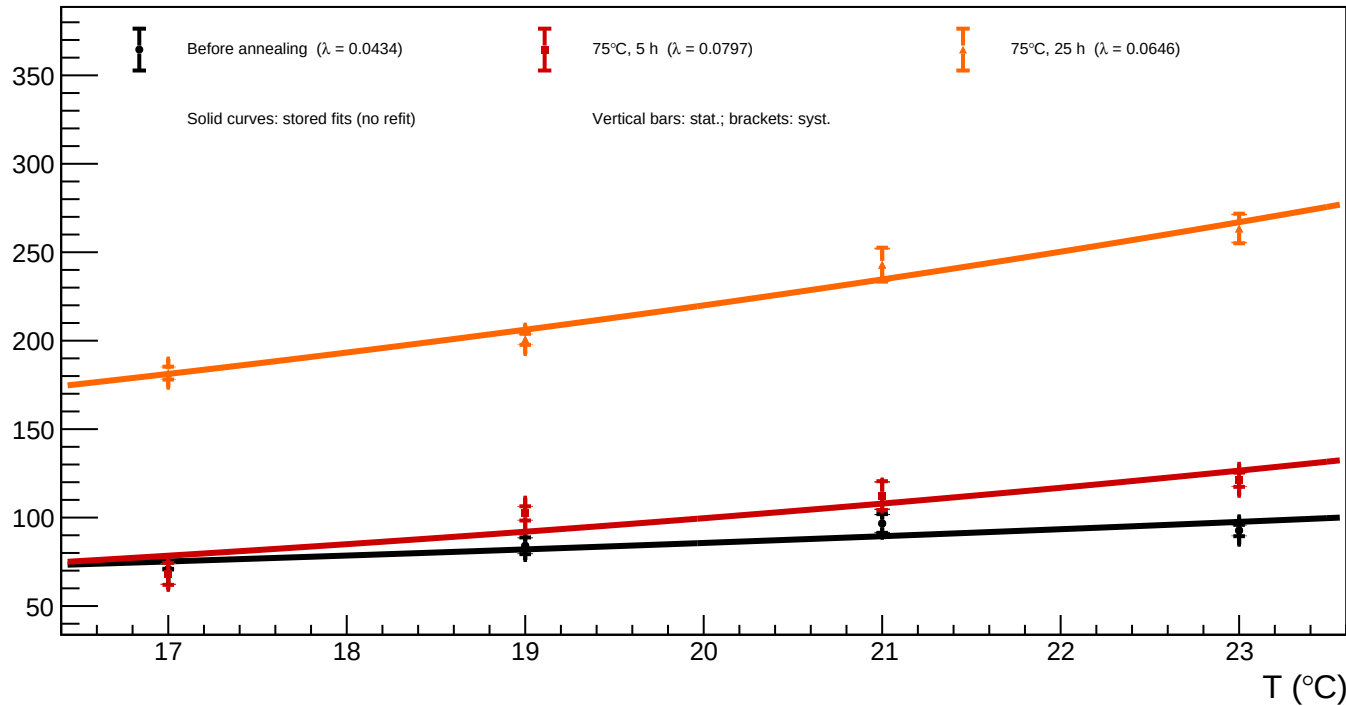
B1_v=3 - Spot 2 (x = 98.20, y = 270.65): luminosity vs temperature for all annealing phases
