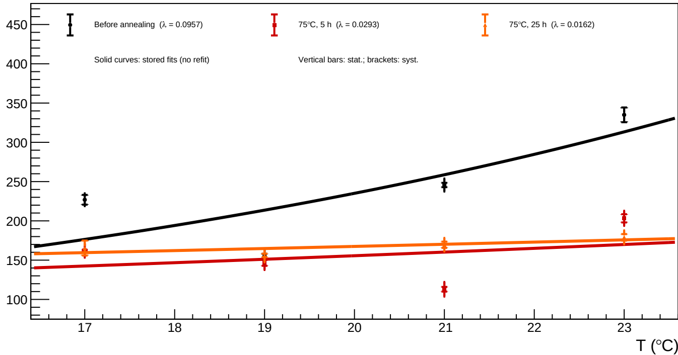
B1_v=3 - Spot 20 (x = 645.38, y = 532.13): luminosity vs temperature for all annealing phases
