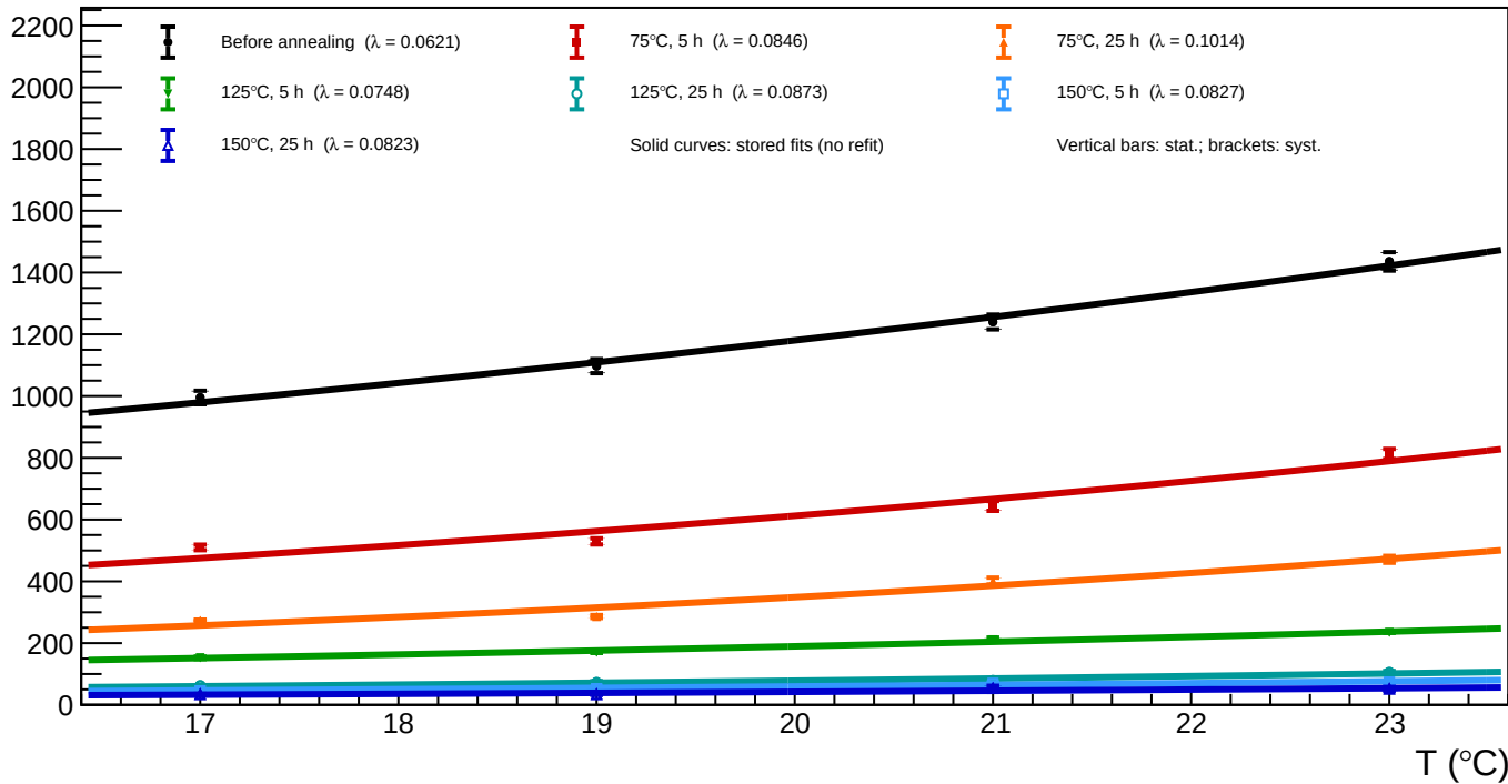
B1_v=3 - Spot 23 (x = 728.64, y = 380.45): luminosity vs temperature for all annealing phases
