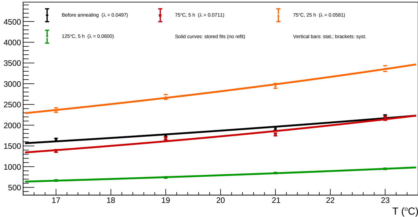
B1_v=3 - Spot 25 (x = 829.77, y = 800.67): luminosity vs temperature for all annealing phases
