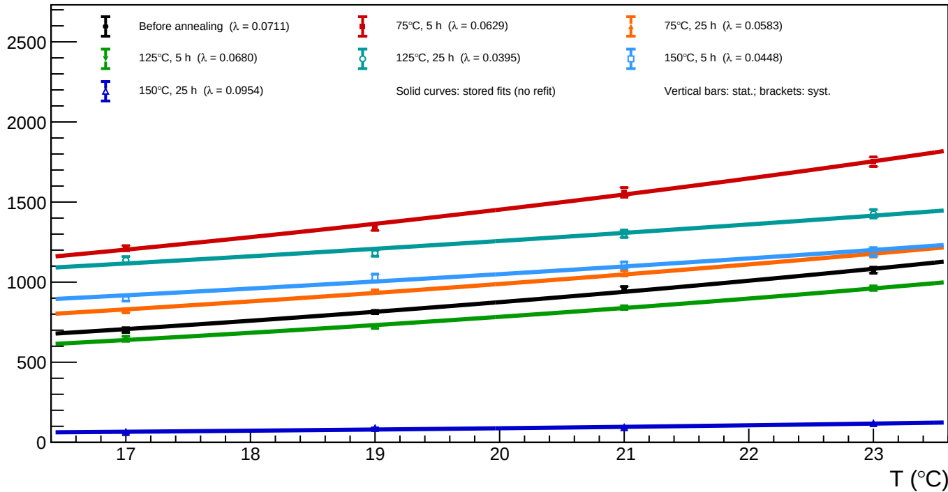
B1_v=3 - Spot 26 (x = 847.68, y = 170.46): luminosity vs temperature for all annealing phases
