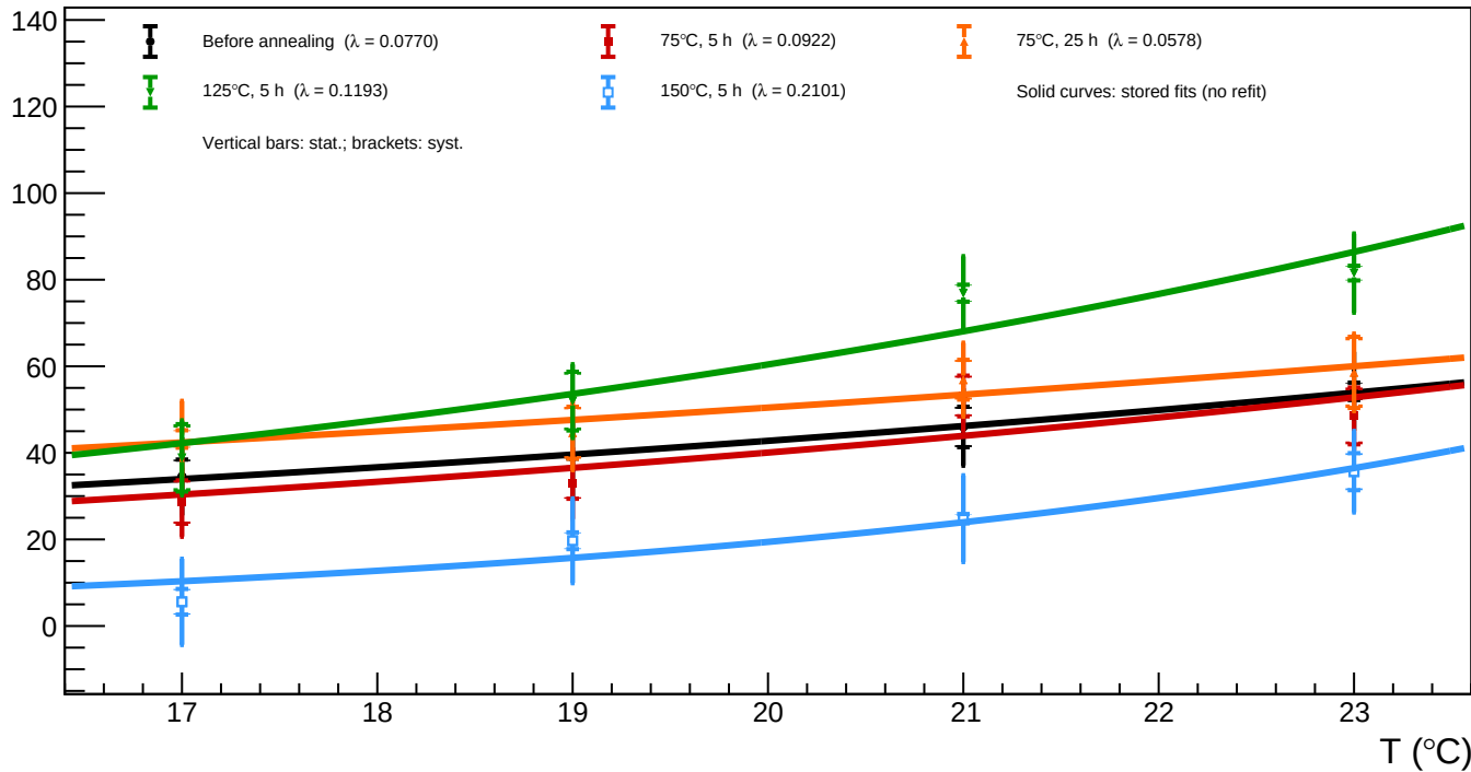
B1_v=3 - Spot 27 (x = 848.40, y = 945.33): luminosity vs temperature for all annealing phases
