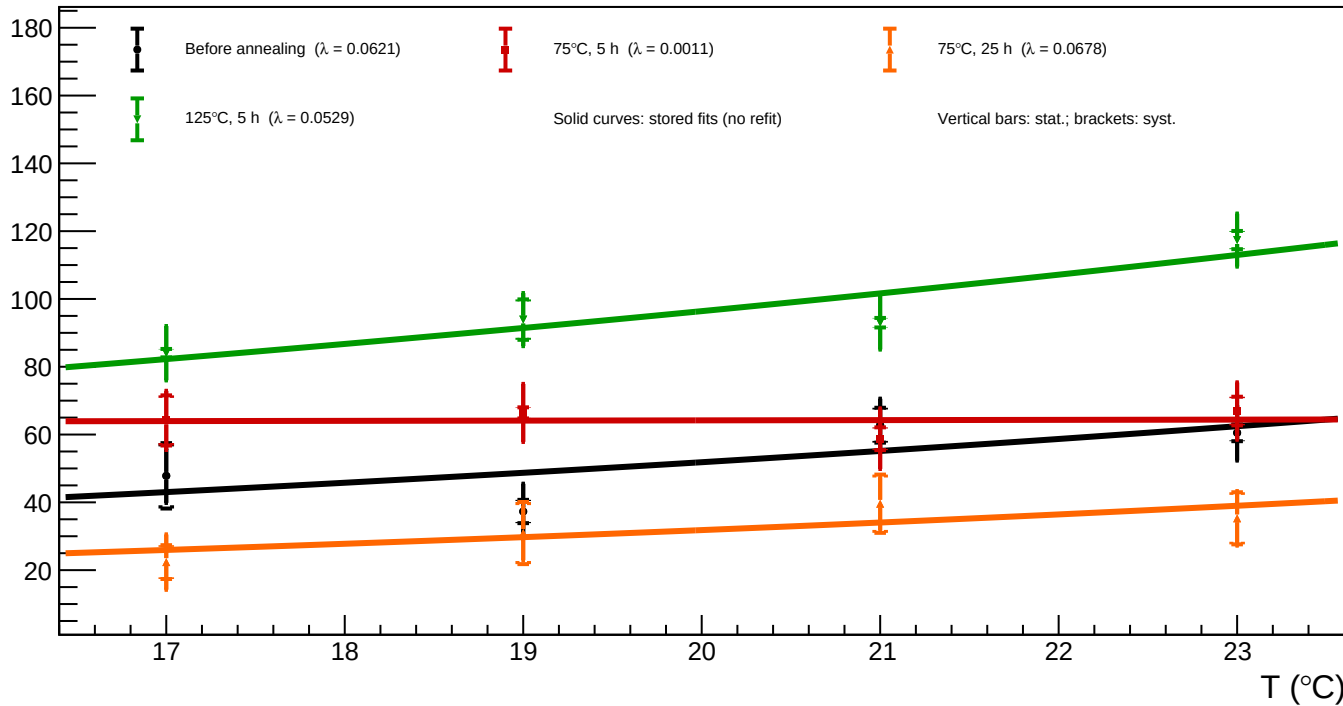
B1_v=3 - Spot 28 (x = 882.46, y = 868.93): luminosity vs temperature for all annealing phases
