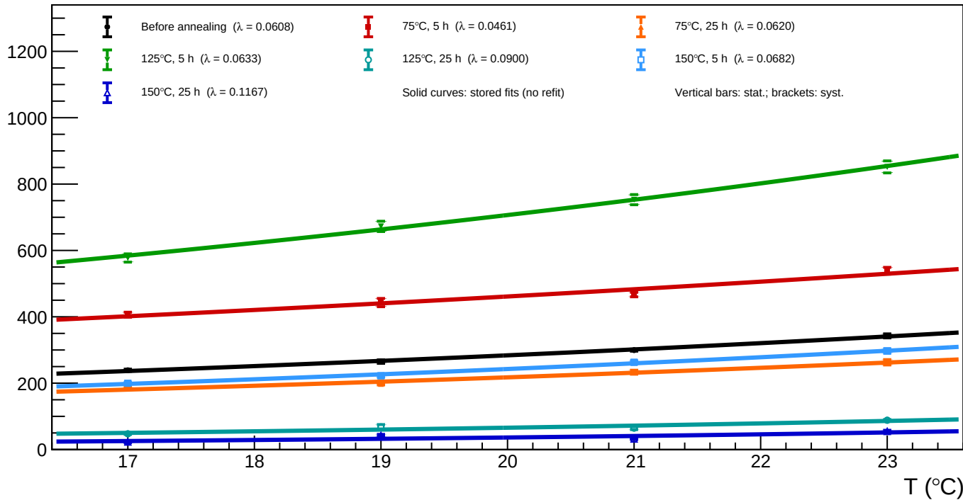
B1_v=3 - Spot 29 (x = 924.72, y = 741.87): luminosity vs temperature for all annealing phases
