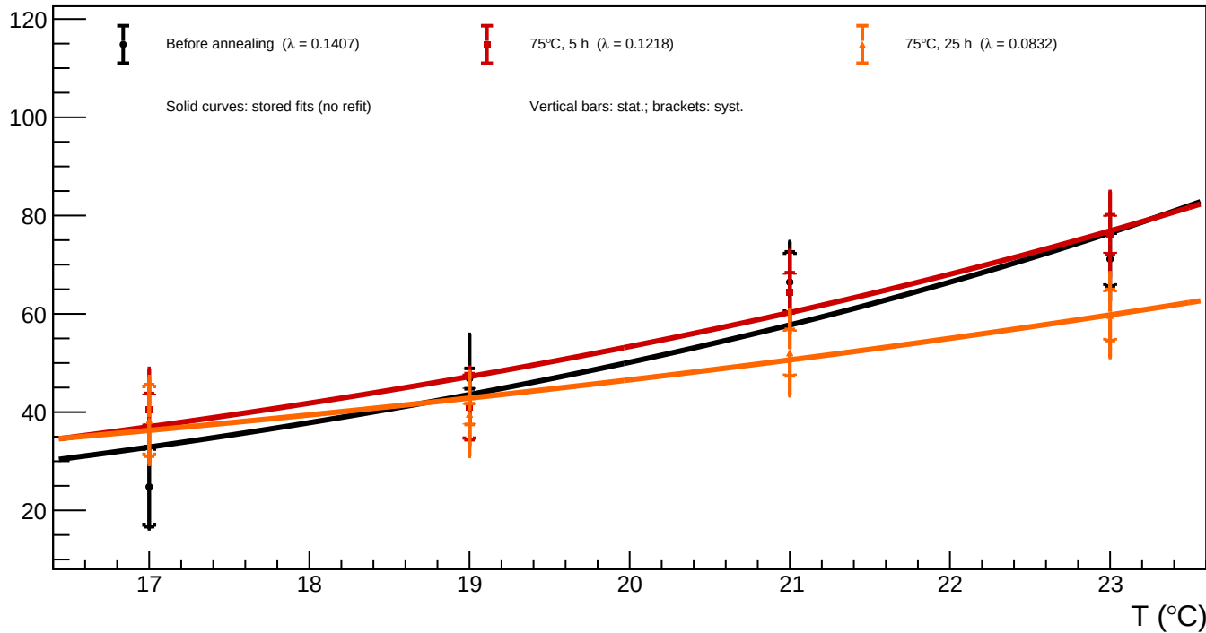
B1_v=3 - Spot 3 ( x = 159.44 , y = 433.10 ): luminosity vs temperature for all annealing phases
