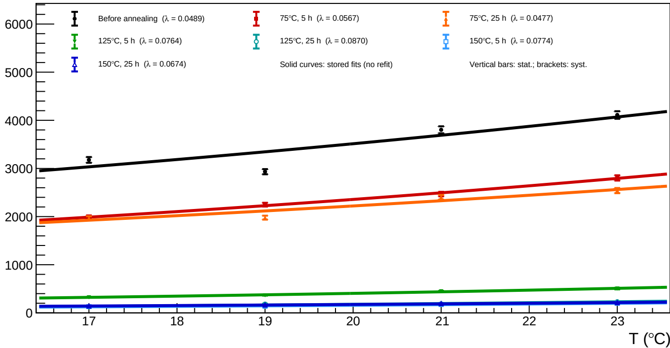
B1_v=3 - Spot 30 (x = 932.58, y = 979.60): luminosity vs temperature for all annealing phases
