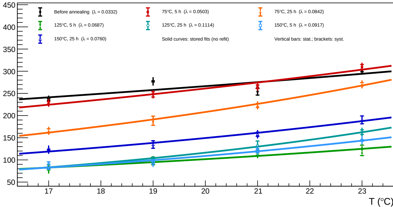
B1_v=3 - Spot 31 (x = 973.13, y = 140.28): luminosity vs temperature for all annealing phases
