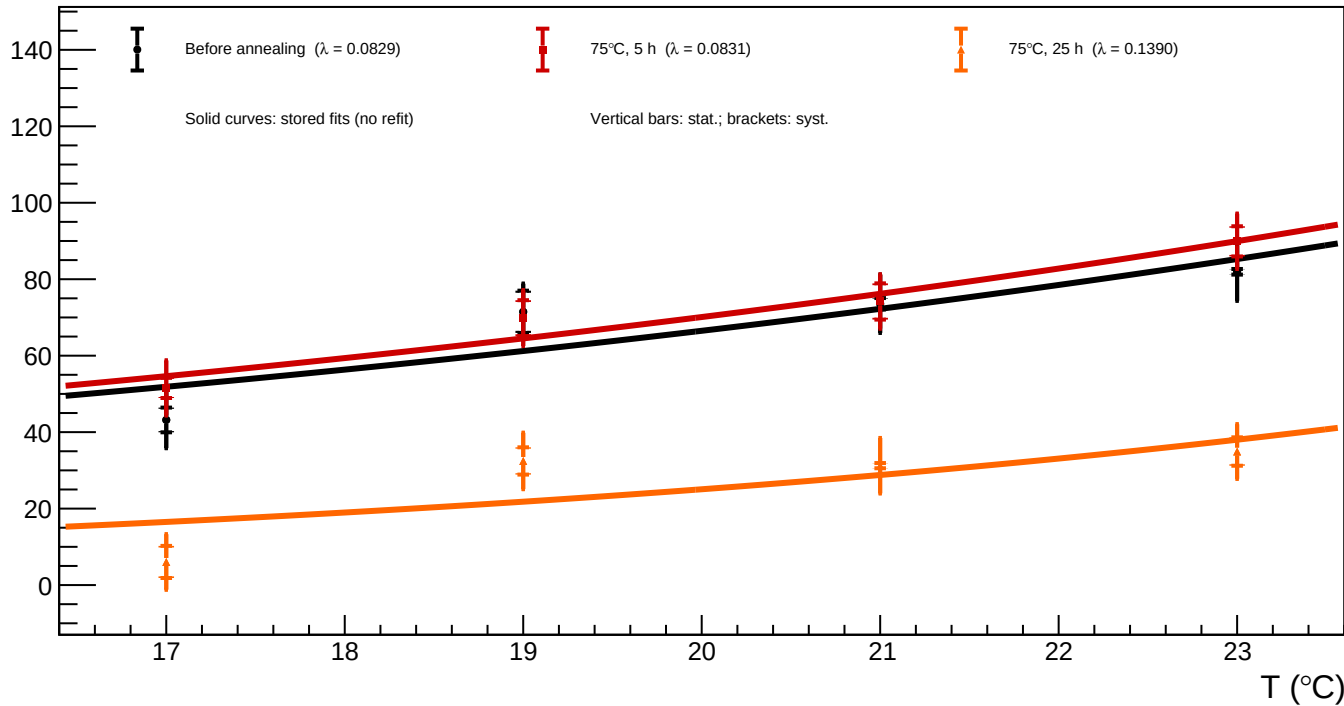
B1_v=3 - Spot 32 (x = 976.60, y = 703.25): luminosity vs temperature for all annealing phases
