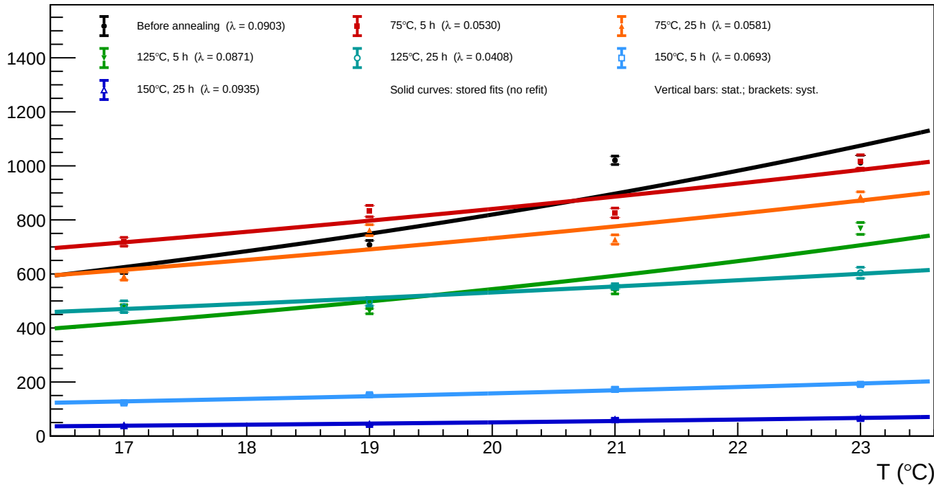
B1_v=3 - Spot 34 ( x = 1067.07 , y = 855.60 ): luminosity vs temperature for all annealing phases
