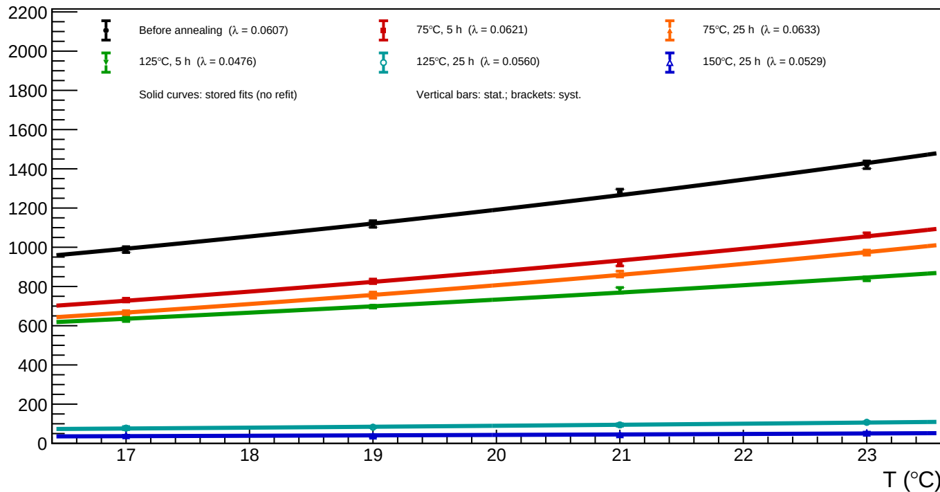
B1_v=3 - Spot 36 ( x = 1109.21 , y = 795.61 ): luminosity vs temperature for all annealing phases
