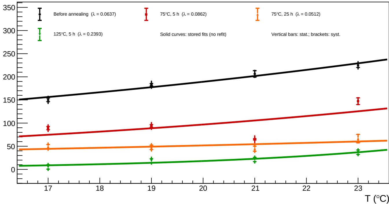
B1_v=3 - Spot 37 (x = 1117.42, y = 919.81): luminosity vs temperature for all annealing phases
