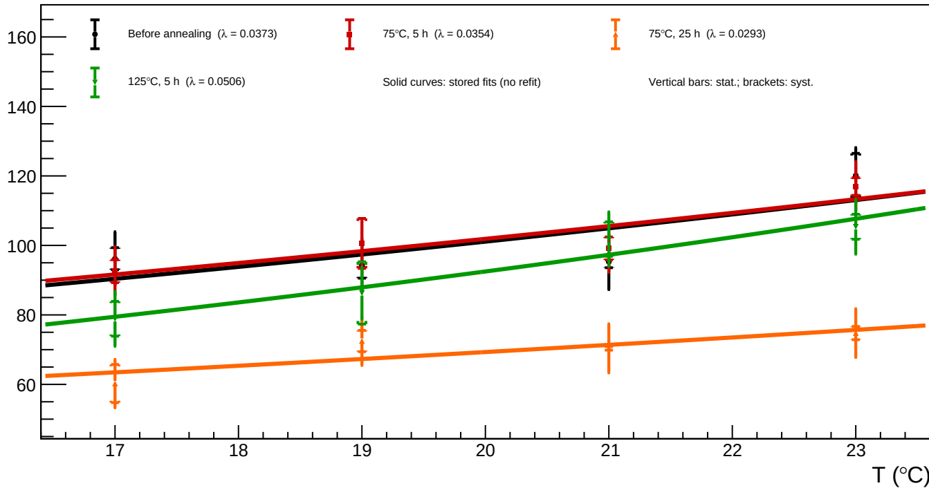
B1_v=3 - Spot 38 (x = 1186.58, y = 759.80): luminosity vs temperature for all annealing phases
