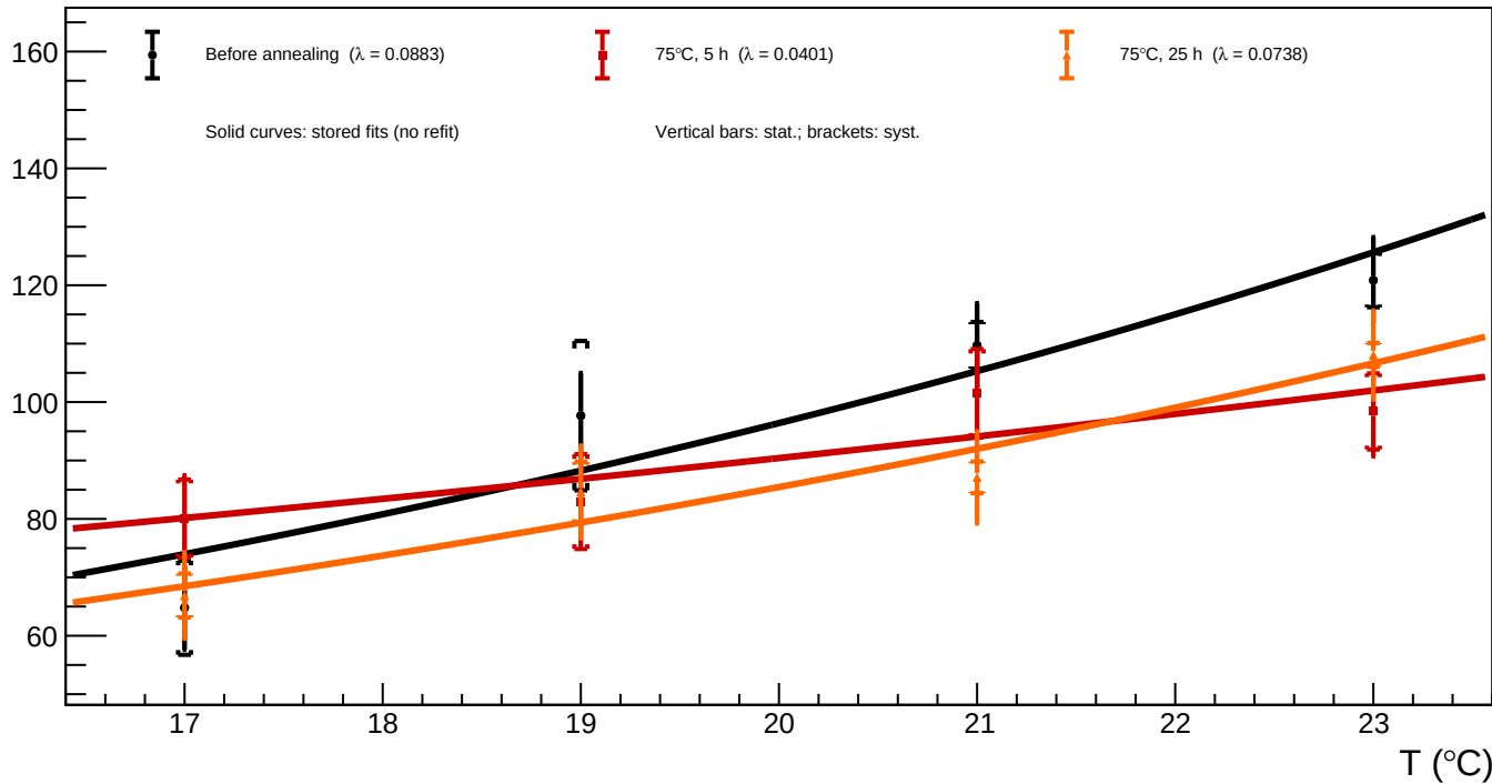
B1_v=3 - Spot 4 (x = 203.07, y = 888.49): luminosity vs temperature for all annealing phases
