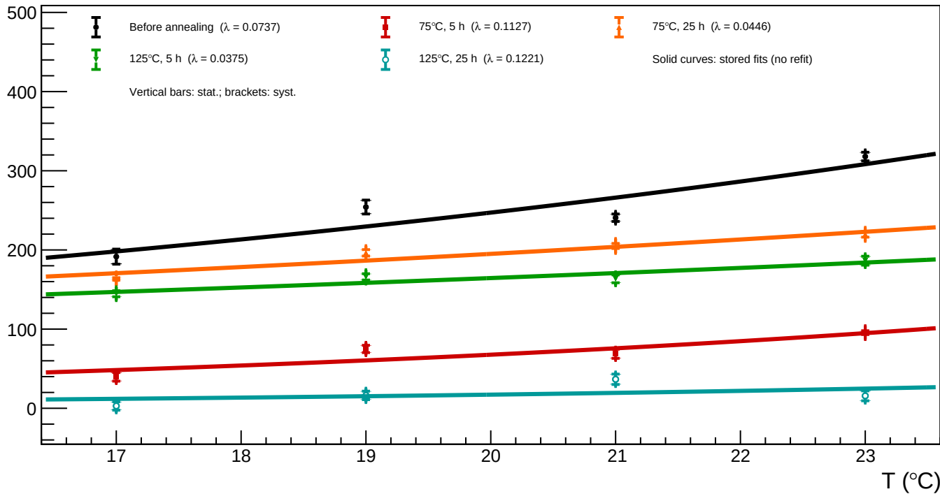
B1_v=3 - Spot 40 (x = 1227.86, y = 82.63): luminosity vs temperature for all annealing phases
