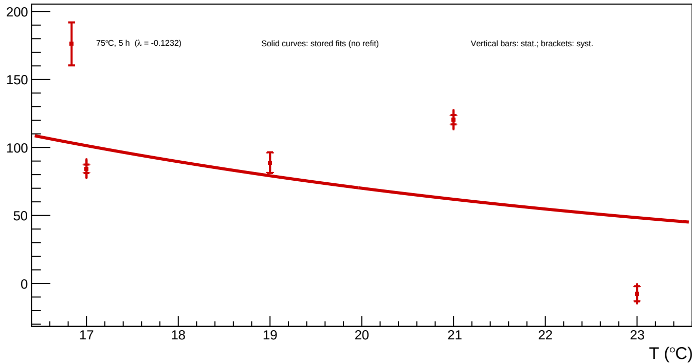
B1_v=3 - Spot 43 (x = 1348.33, y = 135.42): luminosity vs temperature for all annealing phases
