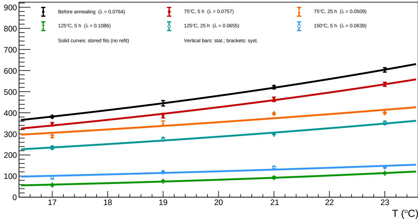
B1_v=3 - Spot 45 (x = 1398.92, y = 769.48): luminosity vs temperature for all annealing phases
