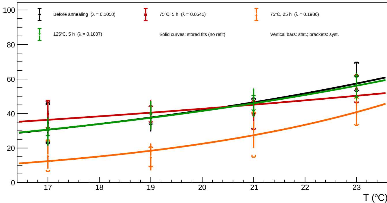
B1_v=3 - Spot 46 (x = 1463.69, y = 878.13): luminosity vs temperature for all annealing phases
