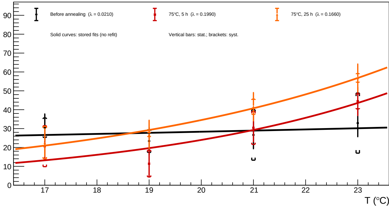
B1_v=3 - Spot 47 ( x = 1498.93 , y = 369.80 ): luminosity vs temperature for all annealing phases
