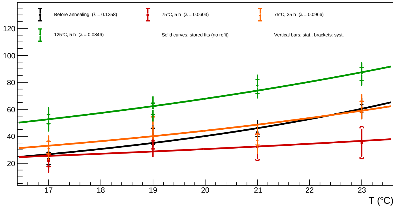
B1_v=3 - Spot 48 (x = 1499.66, y = 981.76): luminosity vs temperature for all annealing phases
