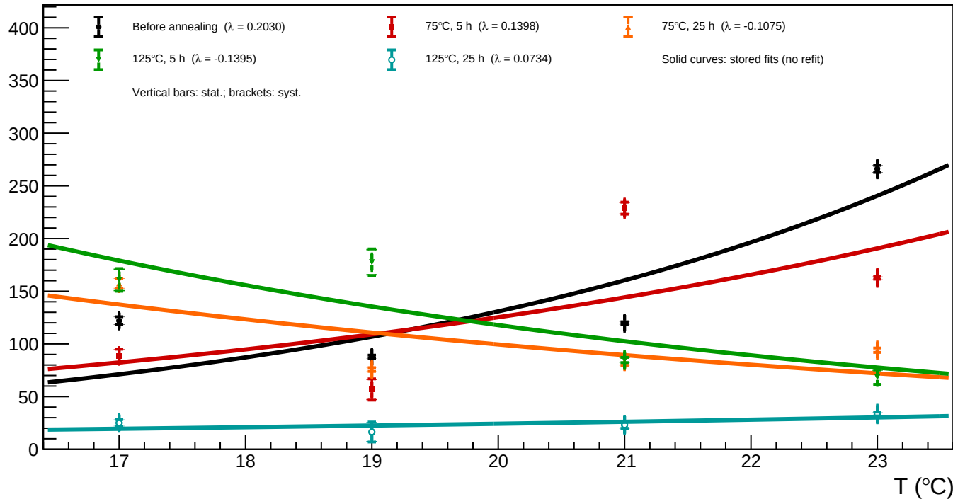
B1_v=3 - Spot 5 ( x = 217.84 , y = 309.86 ): luminosity vs temperature for all annealing phases
