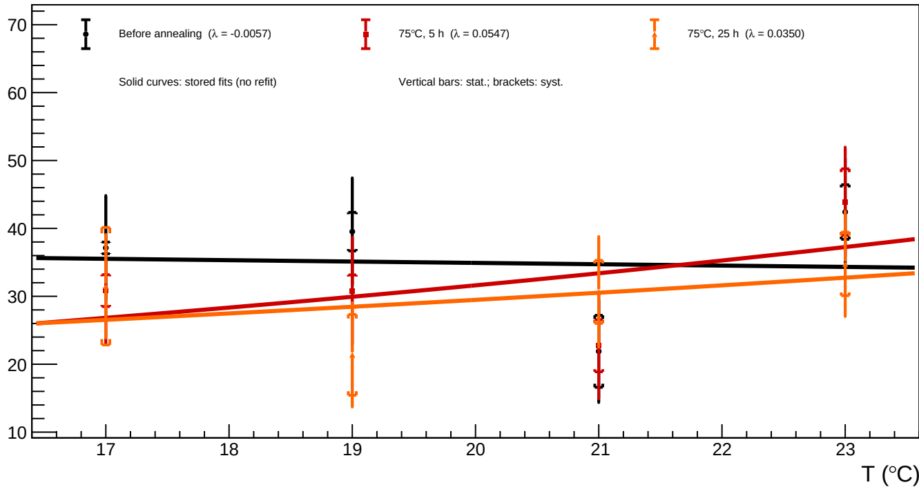
B1_v=3 - Spot 50 ( x = 1556.56 , y = 613.72 ): luminosity vs temperature for all annealing phases
