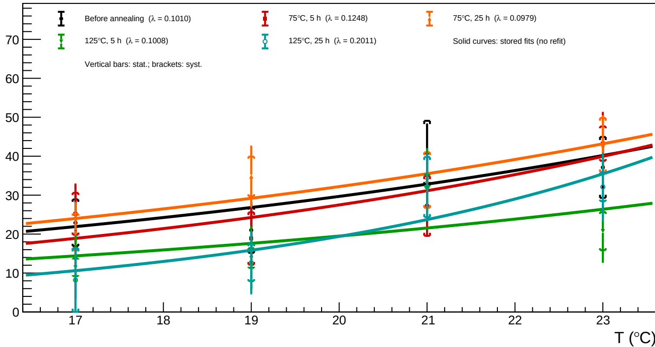
B1_v=3 - Spot 51 ( x = 1587.91 , y = 283.54 ): luminosity vs temperature for all annealing phases
